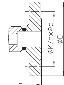
Fig. 682/683/684....1 with flanges
