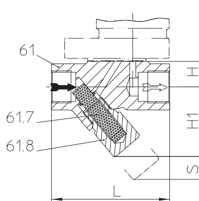
Fig. 682....2 with outside strainer and screwed sockets
