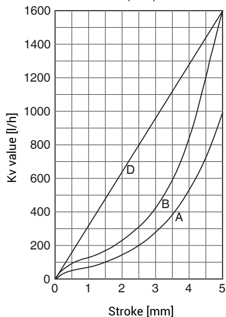
Characteristics DN 10 (seat)
