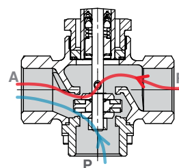
GEMÜ 314 Mixing
