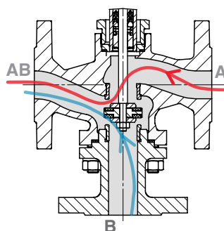
GEMÜ 312 Mixing
