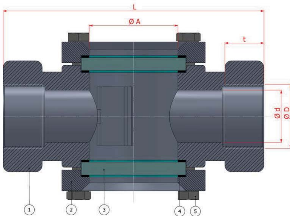
ROSCADA-SCREWED
