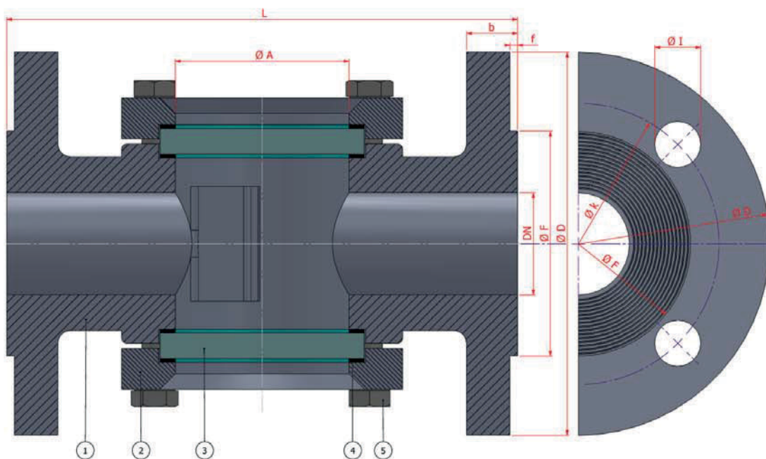
BRIDAS - FLANGED
